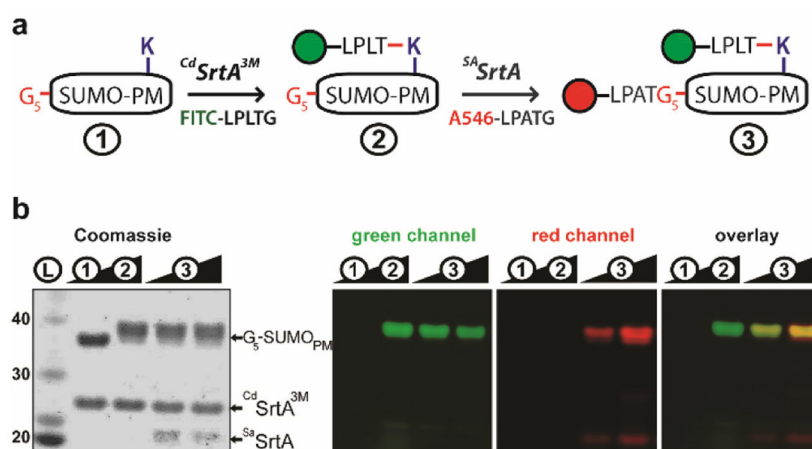
Figure 3. Orthogonal protein labeling using CdSrtA^{3M} and SaSrtA . (A) Sequential reaction scheme used to install fluorogenic peptides on a target protein via peptide- and isopeptide bonds. G_5 -SUMO PM is a SUMO target protein that is fused to N- and C-terminal nucleophiles, pentaglycine ( G_5 ) and the pilin motif (PM), respectively. (B) SDS-PAGE analysis of reaction mixture taken at different steps in the procedure. 1) prior to labeling, 2) after labeling with FITC-LPLTG using CdSrtA^{3M} and 3) after labeling with A546-LPATG using SaSrtA (0.25/2hr incubations). Panels show as indicated fluorescence gel imaging to detect FITC and A546 fluorophores using 488/530 (green channel) and 532/605nm (red channel) wavelengths for excitation/emission, respectively, and the merged image of the gels demonstrating dual labeling. In the first panel, the same gel was visualized by coomassie staining.
