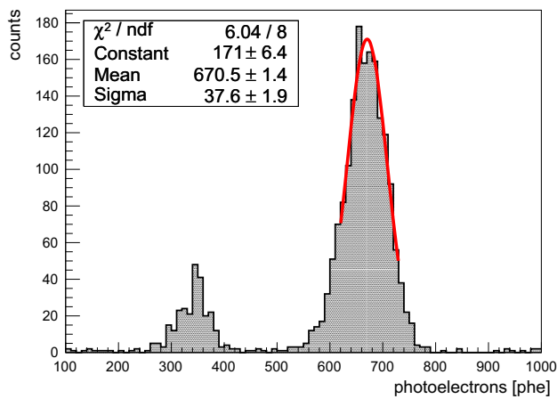
Fig. 3 NaI-33 calibration spectrum with 241 Am source. The gaussian fit to the 59.5 keV peak is shown in red
