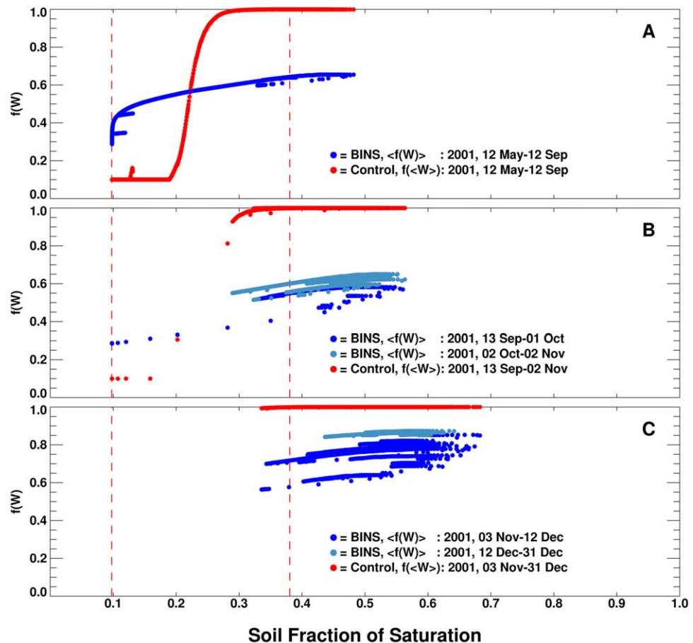
Figure 10. Soil moisture stress at BR-PEG as a function of root-weighted soil moisture for the SiB3 control run (red) and SiB3-Bins run (blue), for the period 12 May to 31 December 2001. (a) Drying period, 12 May to 12 September, when there is little or no rain. (b) Rapid moistening in the last 2 weeks of September. (c) Further moistening in November and December.
