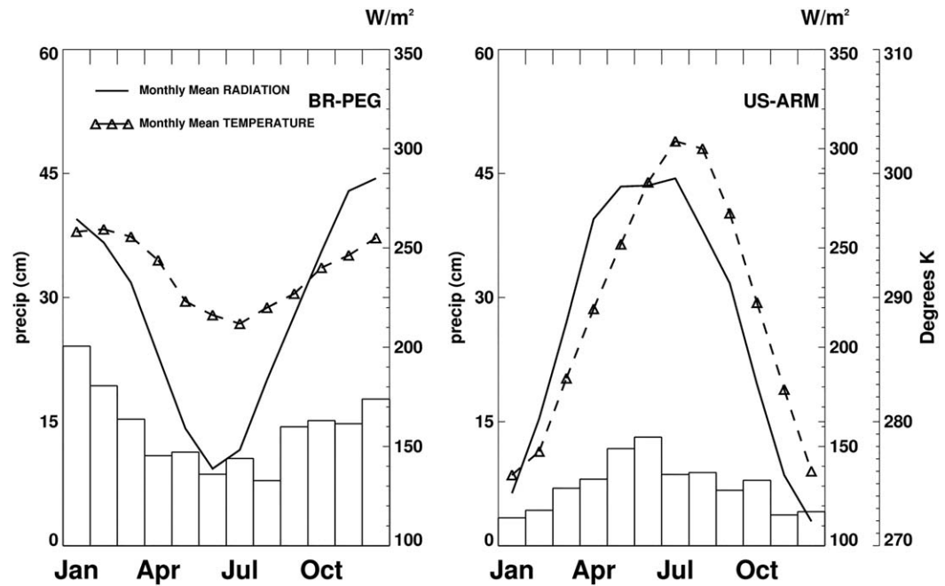
Figure 4. Mean annual cycle of precipitation, radiation, and temperature for the (a) BR-PEG and (b) US-ARM tower sites.
