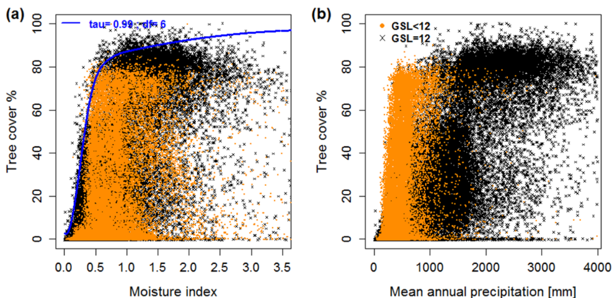
Figure 7. (a) Global tree cover versus moisture index (MI, average growing season moisture); (b) Global tree cover versus mean annual precipitation. Black points represent sites with growing season length (GSL) of 12 months (approximately tropical and subtropical regions with latitudes \leq 40^\circ N and S) and orange points represent sites with GSL < 12 months. There is a more cohesive pattern of tree cover when MI is used instead of precipitation. (a) shows the non-parametric 0.99 quantile regression line.
