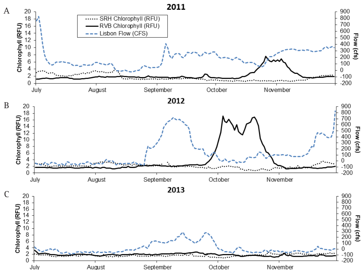
Figure 5 Chlorophyll- a concentration, measured as relative fluorescence units (RFU), in the Sacramento River at Hood (SRH; just south of Freeport; see Figure 1) and the Sacramento River at Rio Vista (RVB) in relation to flow in cubic feet per second (cfs) through Yolo Bypass measured at Lisbon Weir (Lisbon Flow)
