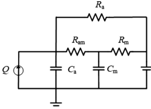
Fig. 2 Example of a 3R2C thermal circuit building model. The subscript a represents indoor air temperature, while m represents the building mass. Q represents the combined heat input from the heat pump and indoor loads.
