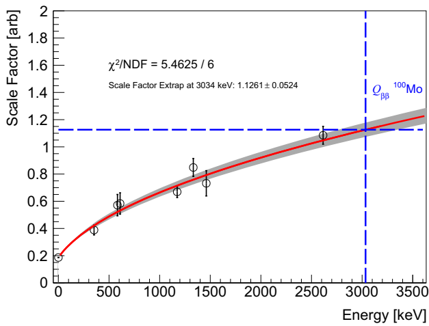
Fig. 11 Resolution scaling fit showing the scaling factor R , between background and calibration data for each peak in physics data. We model this as R(E) = \sqrt{p_0^2 + p_1 E} and extrapolate to Q_{\beta\beta} to obtain a global scale factor. The choice of functional form derives from the energy resolution scaling in data following this same functional form
