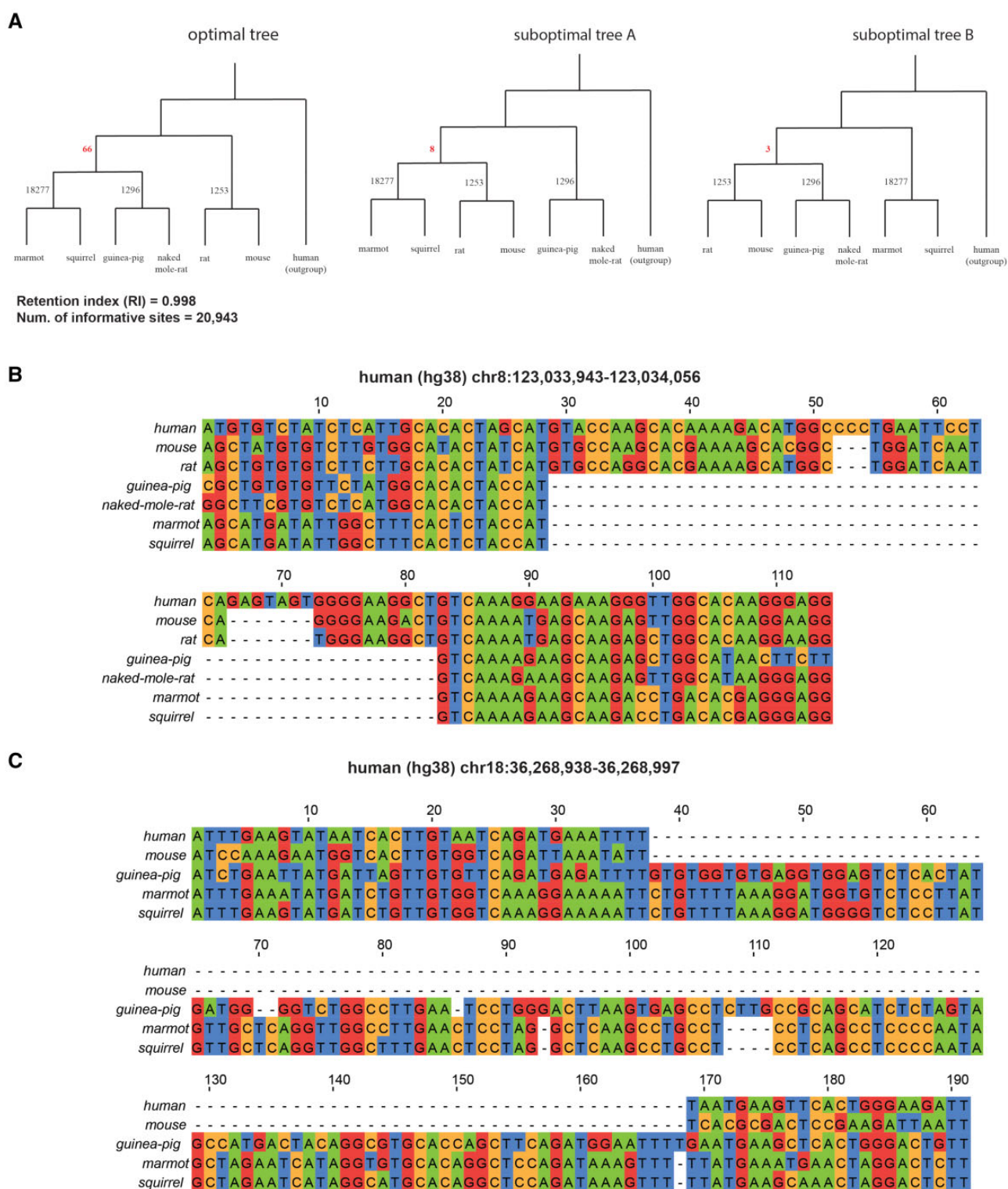
FIG. 3. —Champagne places Myomorpha sister to Sciuridae and Hystricomorpha (A) The maximum parsimony tree generated by PAUP* using Champagne's character matrix for a subset of rodents (left), alongside two less parsimonious trees that reflect alternate branching relationships between Sciuridae, Myomorpha, and Hystricomorpha. Sixty-six indels support Myomorpha as the sister clade, whereas only 8 and 3 support the other alternatives. (B) A multiple sequence alignment for a 54-bp deletion shared by guinea pig, naked mole rat, marmot, and squirrel. (C) A multiple sequence alignment for a 125-bp insertion shared by guinea pig, marmot, and squirrel.
