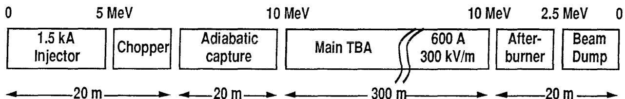
Fig. 2. Layout of one RK-TBA unit
