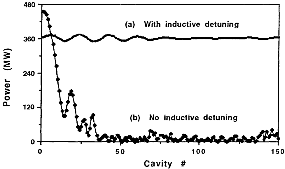
Fig. 5. Power extraction from 150-cavities in one unit of RK-TBA: (a) with inductive detuning ( \Delta^- = 30^\circ , phase velocity 1.33c); (b) no inductive detuning ( \Delta^- = 0^\circ , phase velocity 1.0c).
