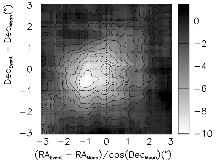
Figure 1: Two dimensional plot of the moon shadow. The background was calculated using the time-slicing method (Alexandreas et al., 1993). The data and background maps were then smoothed with square bins 2.1^\circ on a side. The significance was calculated by the method of Li & Ma (Li & Ma, 1983). The circle shown is of radius 0.26^\circ and is centered at the undeflected position of the moon.
