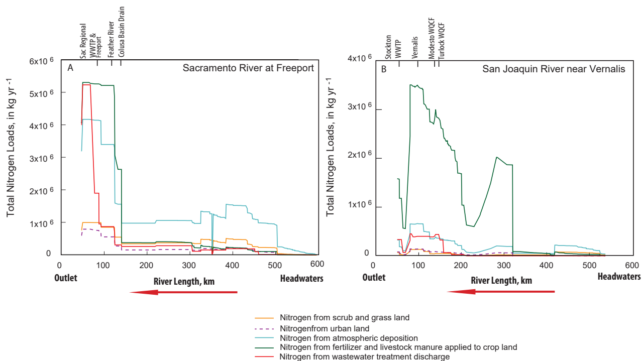
Figure 13 Annual nitrogen loads from various sources in kilograms upstream of the (A) Sacramento River at Freeport and (B) the San Joaquin River near Vernalis from the 2012 SPARROW model
