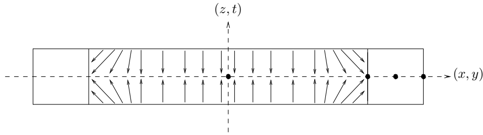
Figure 12: The projection \pi: \partial W \rightarrow B \cup C \cup F
