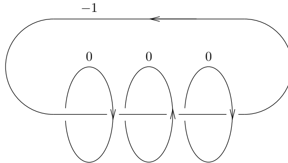
Figure 13: \psi^{-1}(0, 0, -1) , in the case of two elliptic anticomplex points and one hyperbolic anticomplex point
