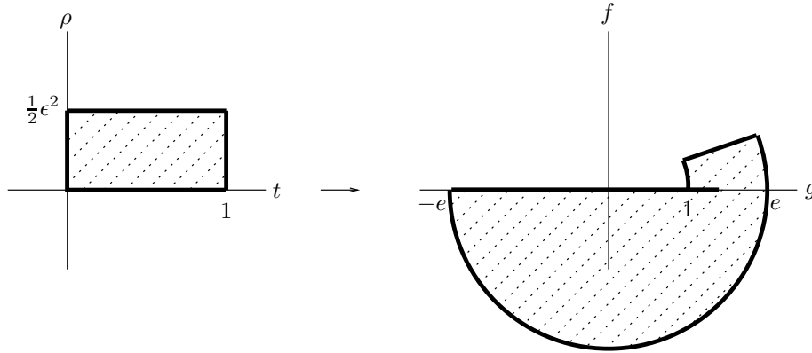
Figure 10: The map \phi
