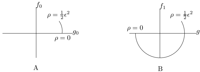
Figure 9: Graphs of \rho \mapsto (g_0(\rho), f_0(\rho)) and \rho \mapsto (g_1(\rho), f_1(\rho))
