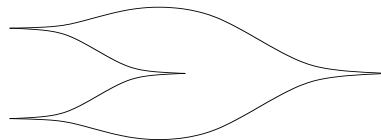
Figure 3: Knot with (\text{tb}, \text{rot}) = (-2, \pm 1)
