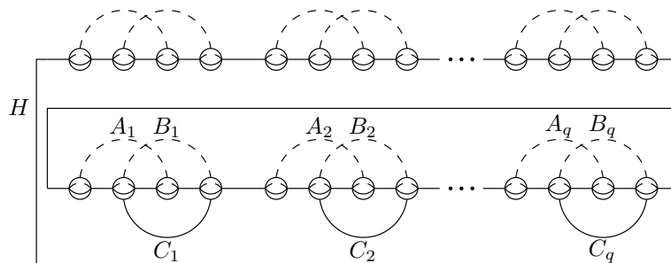
Figure 6: Handlebody decomposition of W'
