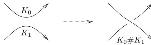
Figure 2: Connected sum of Legendrian knots
